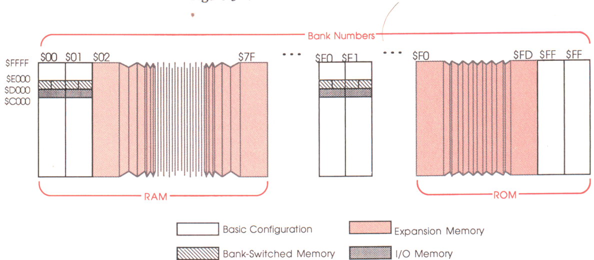
Figure 3-1 Apple IIGS memory map
